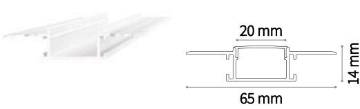
PROFILE 20 mm
